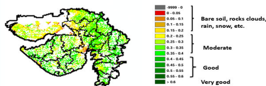
NOAA/VIIRS/BLENDED NDVI Composite ending on Week no 42 ( 15.10.2025 to 22.10.2025) over Agricultural region Gujarat
