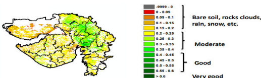
NOAA/VIIRS/BLENDED NDVI Composite ending on Week no 11 (12.03.2025 to 18.03.2025) over Agricultural region
