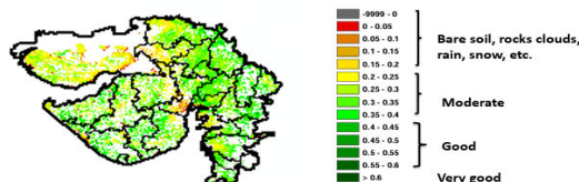
NOAA/VIIRS/BLENDED NDVI Composite ending on Week no 42 ( 15.10.2025 to 22.10.2025) over Agricultural region Gujarat
