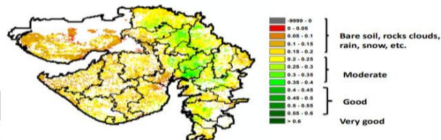
NOAA/VIIRS/BLENDED NDVI Composite ending on Week no 13 (26.03.2025 to 01.04.2025) over Agricultural region
