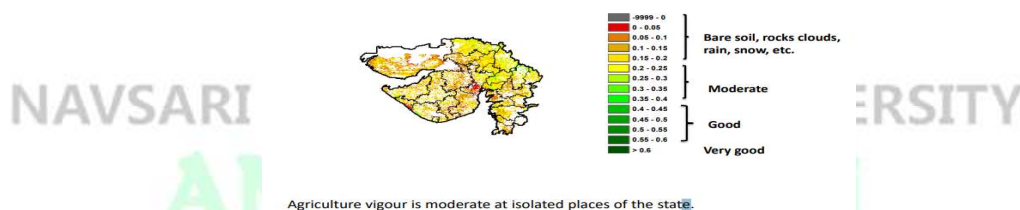
NOAA/VIIRS/BLENDED NDVI Composite ending on Week no 34 ( 20.08.2025 to 26.08.2025) over Agricultural region Gujarat
